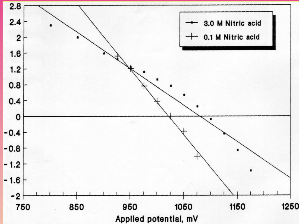
Fig. 4. Test of equation of wave of 6.0 \times 10^{-5} M Meta-Hydroxyacetanilide in Nitric acid medium; Experimental points from Fig. 2.
