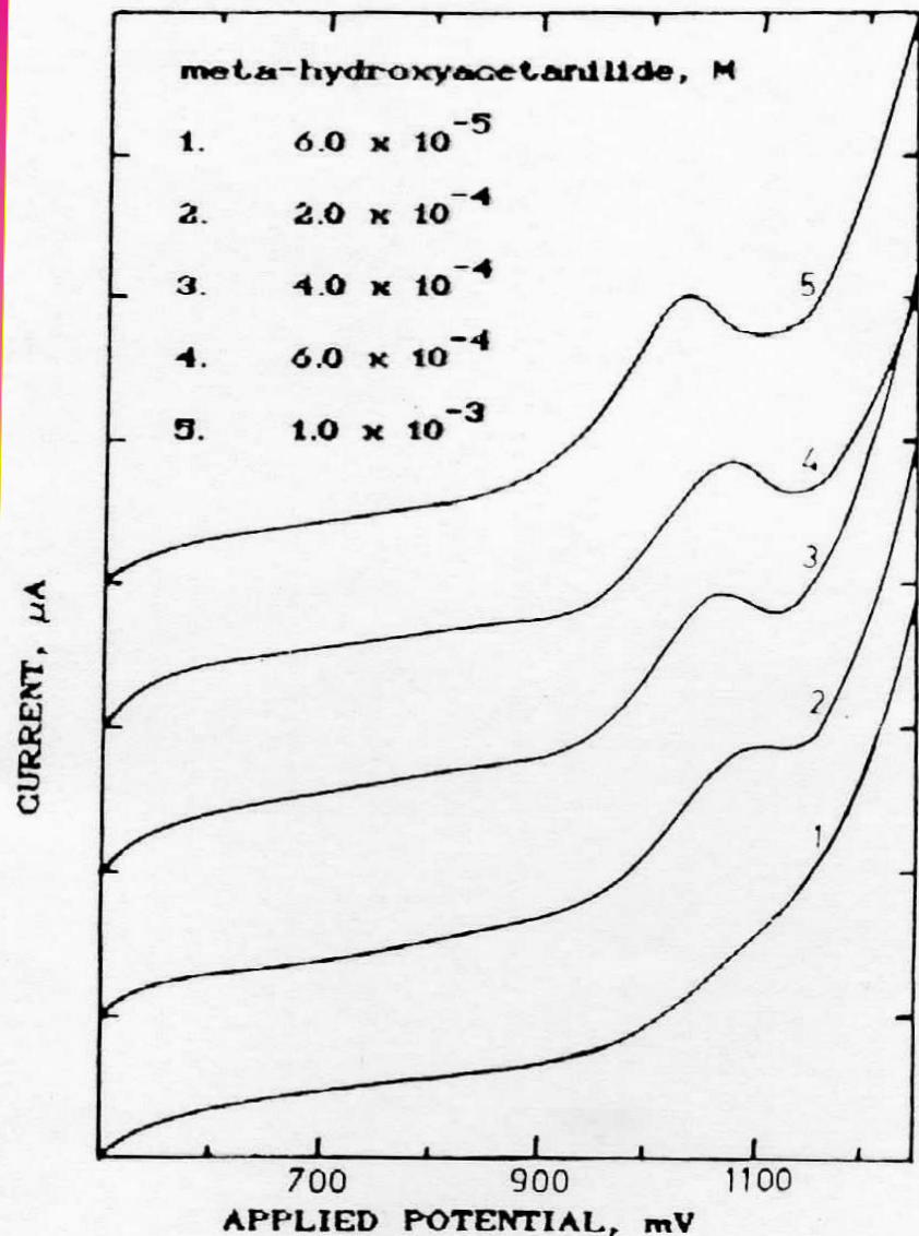
Fig. 3. Calibration polarogram for meta-hydroxyacetanilide determination in 0.1 M HNO 3
