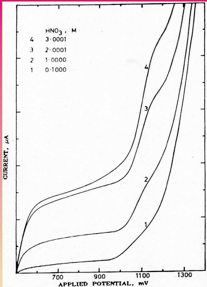
Fig. 2. Effect of HNO 3 concentration on the anodic wave of 6.0 \times 10^{-5} M meta-hydroxyacetanilide
