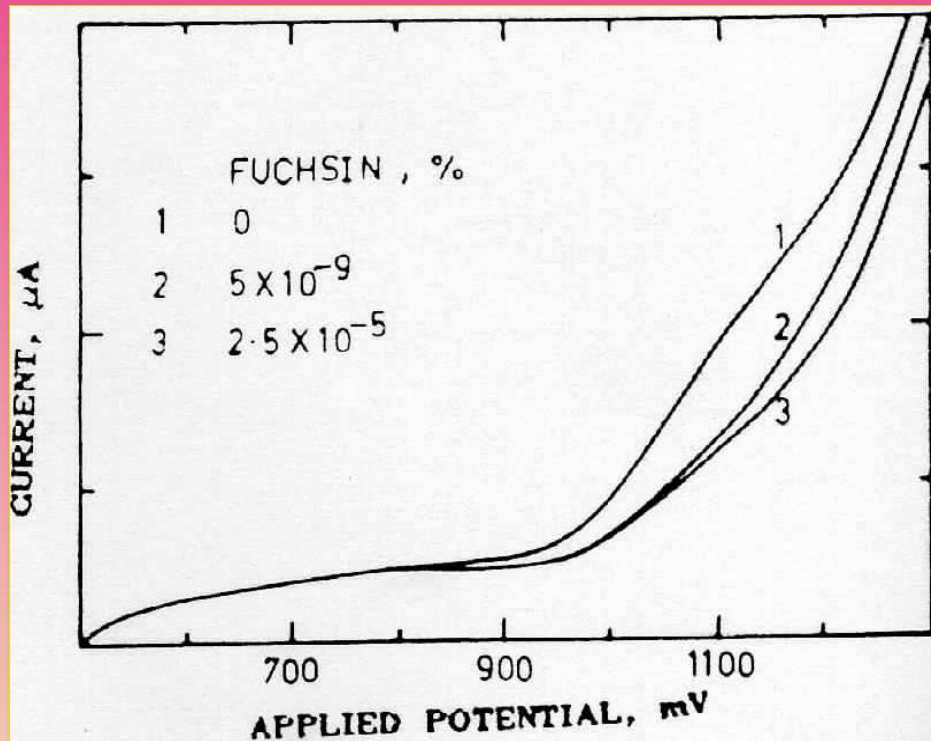
Fig . 1. Effect of Fuchsin concentration on the anodic wave of 6.0 \times 10^{-5} M meta-hydroxyacetanilide in 0.1 M HNO 3
