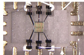
Nanocrystalline Tin Oxide NOx and CO Sensor
